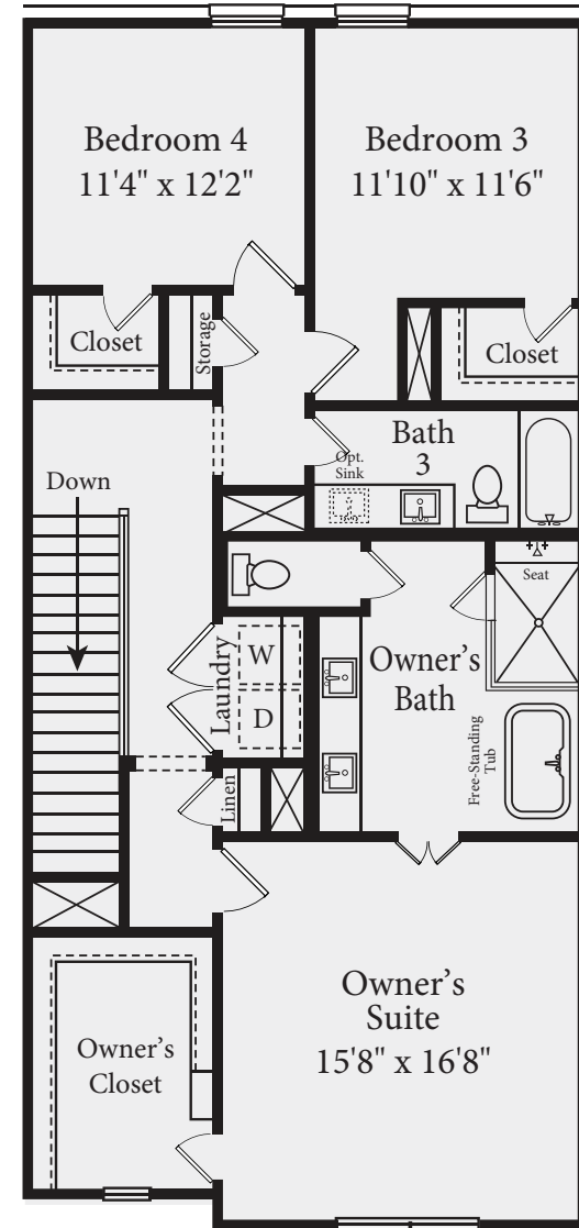
THIRD FLOOR
